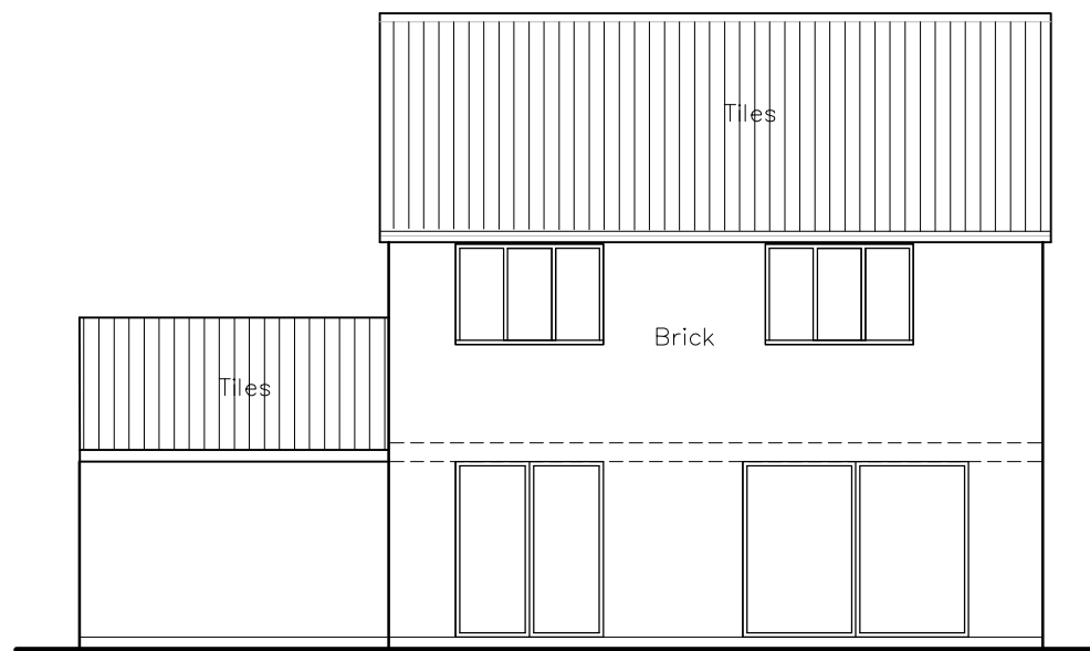
WEST ELEVATION
