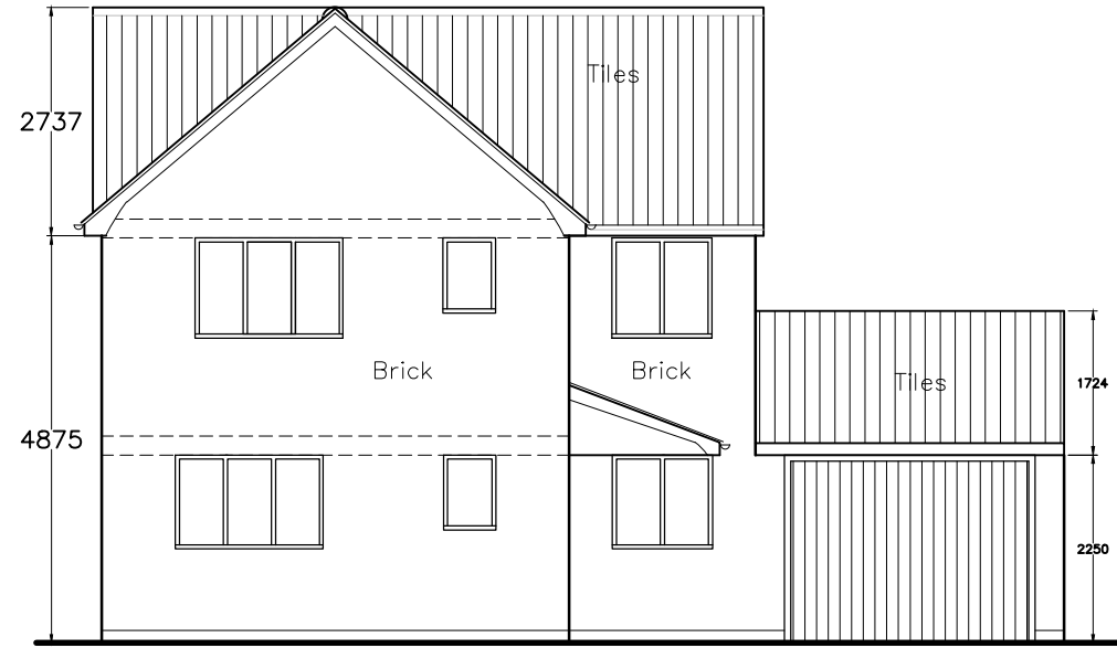
EAST ELEVATION
